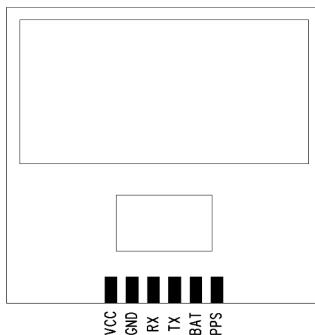
Figure 2: SKM52 Bottom View
