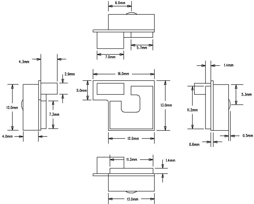
Figure 3: SKM56-J Dimensions
