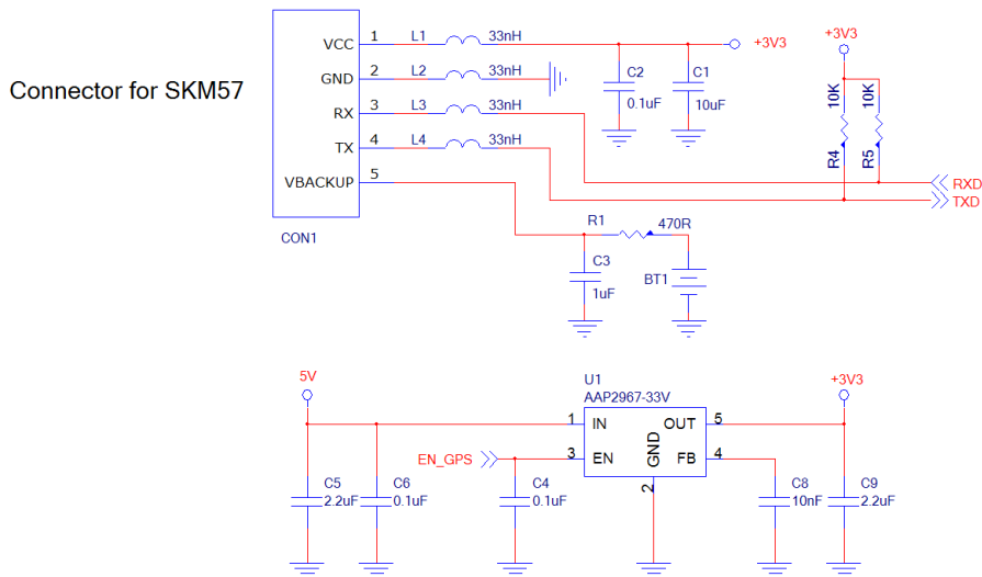
Figure 5: SKM56-J Typical Reference design schematic
