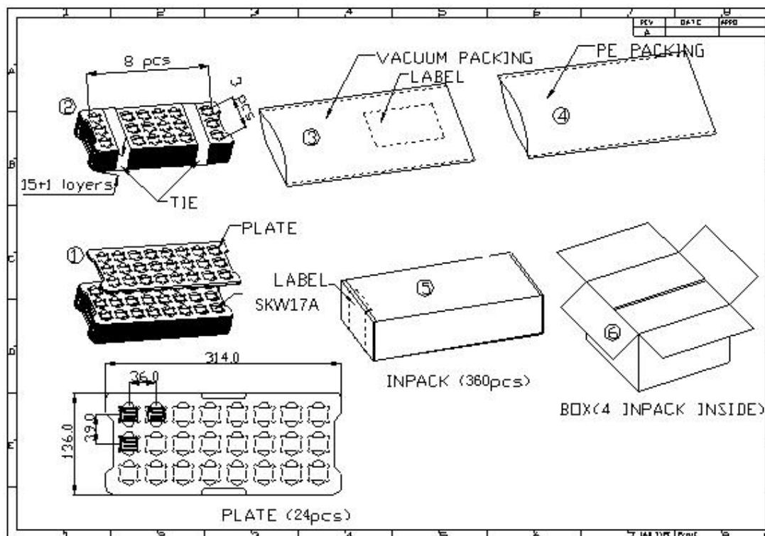
Figure 7: SKW17A Packaging
