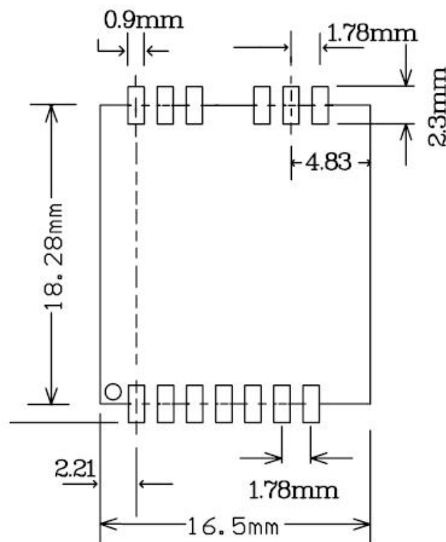
Figure 4: SKW17A Dimensions
