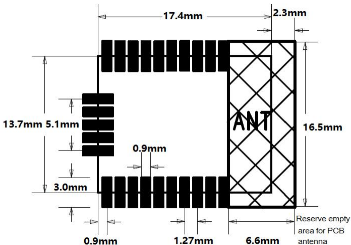
Figure 8 SKB376 Recommended PCB Footprint
