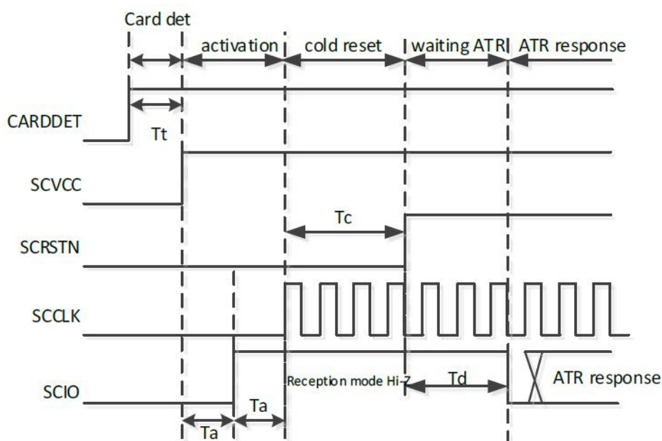
Figure 6-21 Activation, Cold Reset and ATR
