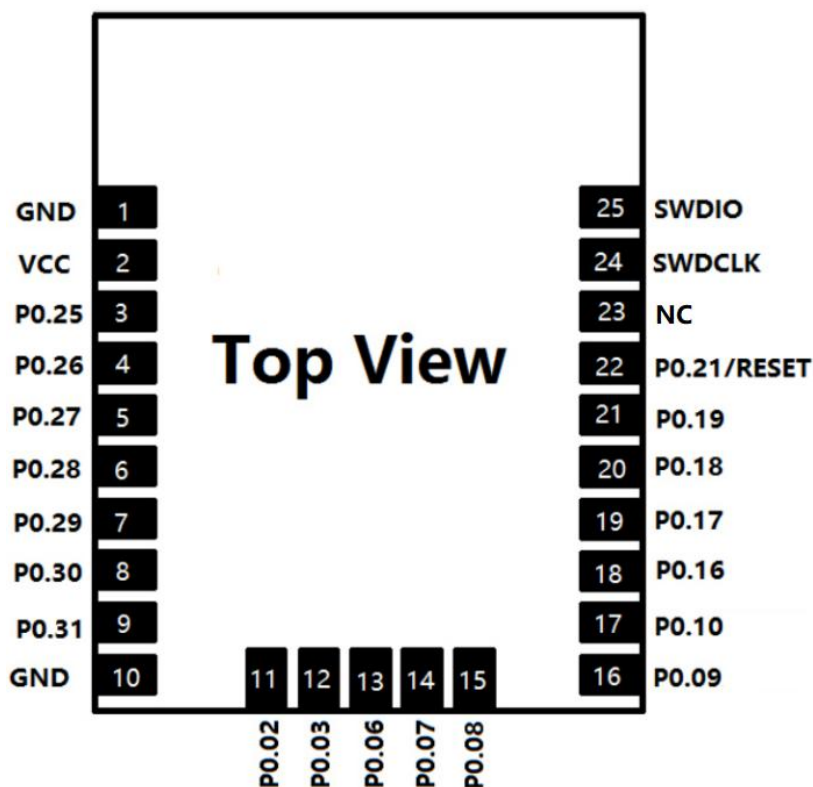
Figure 5: SKB376 Module Pinout
