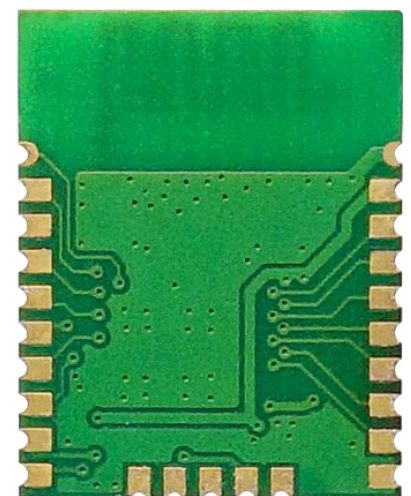
Figure 3-2: SKB376 bottom side
