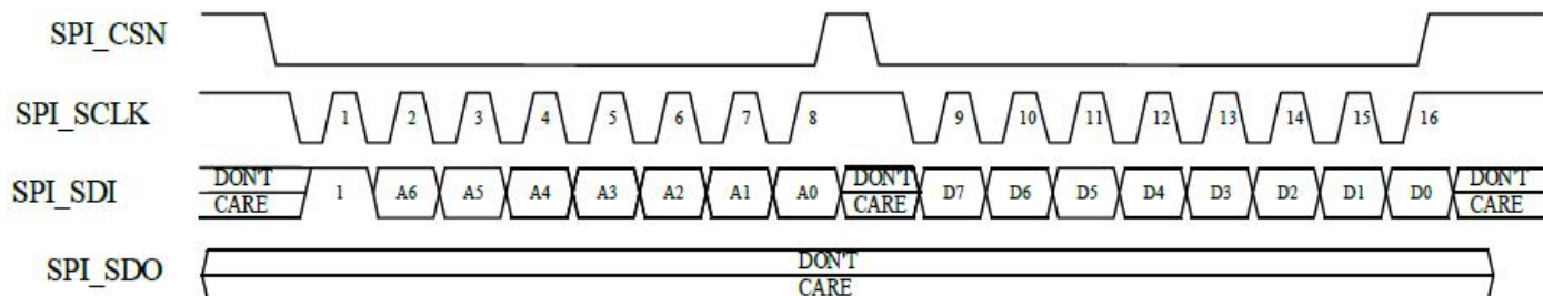
Figure 6-8 4-wire SPI write operation
