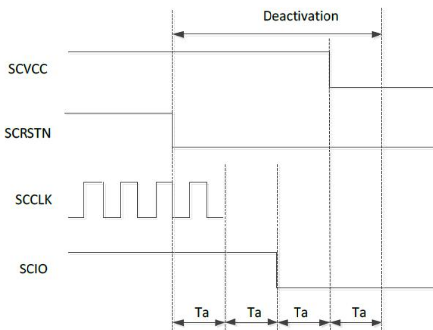
Figure 6-22 Deactivation Sequence
