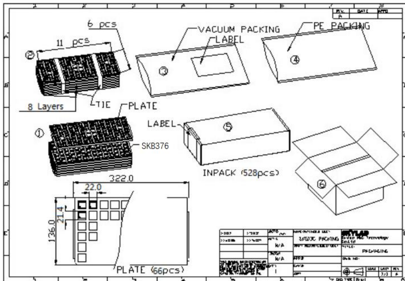
Figure 11: SKB376 Packaging
