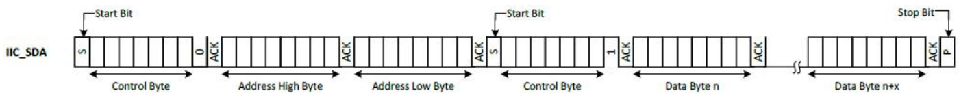
Figure 6-6 I2C sequential read format
