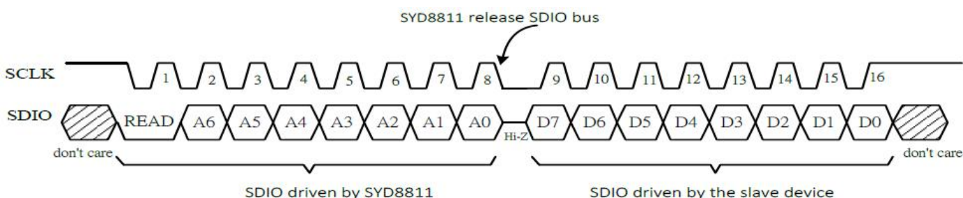
Figure 6-11 3-wire SPI read operation
