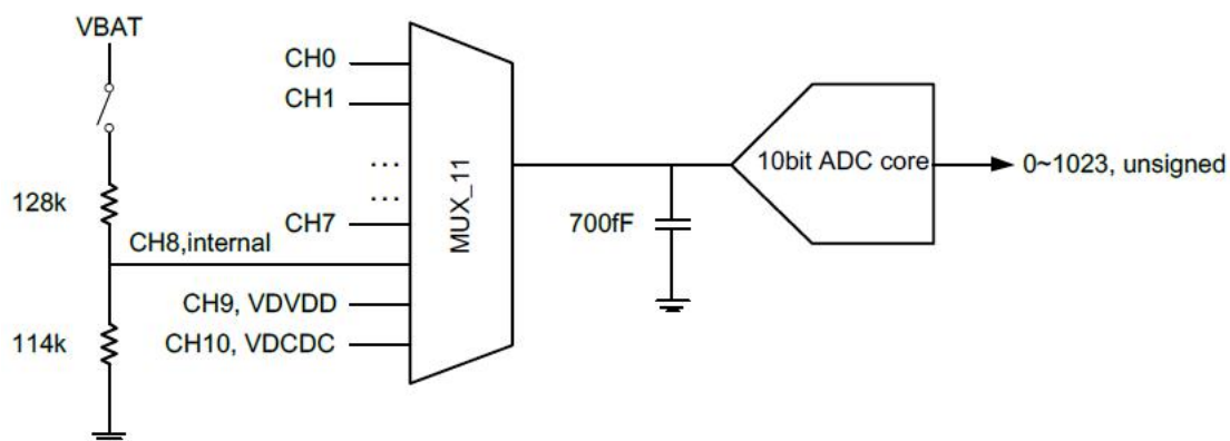
Figure 6-14 GPADC input channel select and VBAT resistance divider configuration
