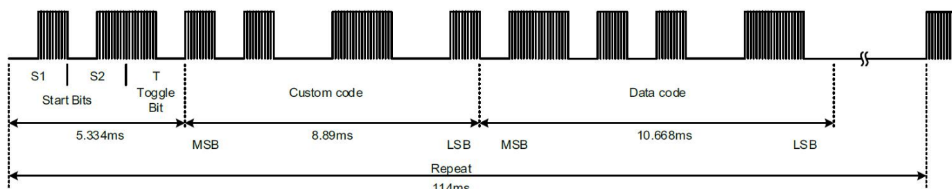
Figure 6-24 RCS5 coded wave format
