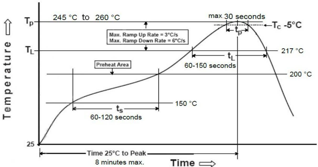
Figure 5: SKZ306 Typical Lead-free Soldering Profile
