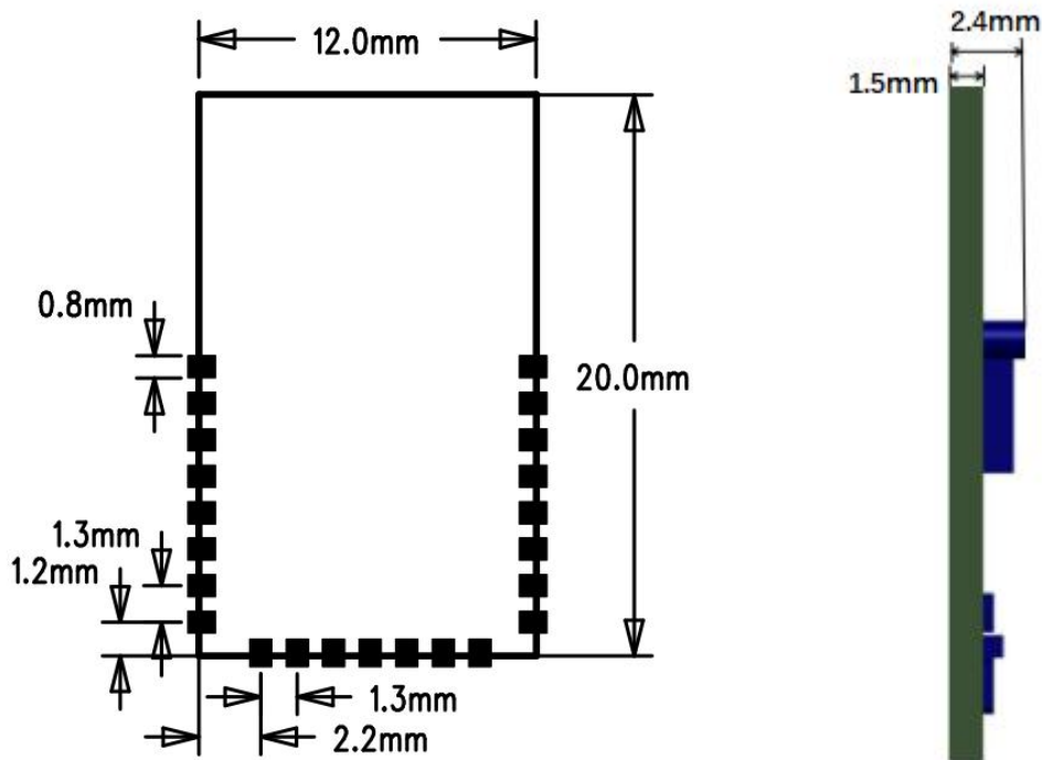
Figure 4 SKZ306 Recommended PCB Footprint
