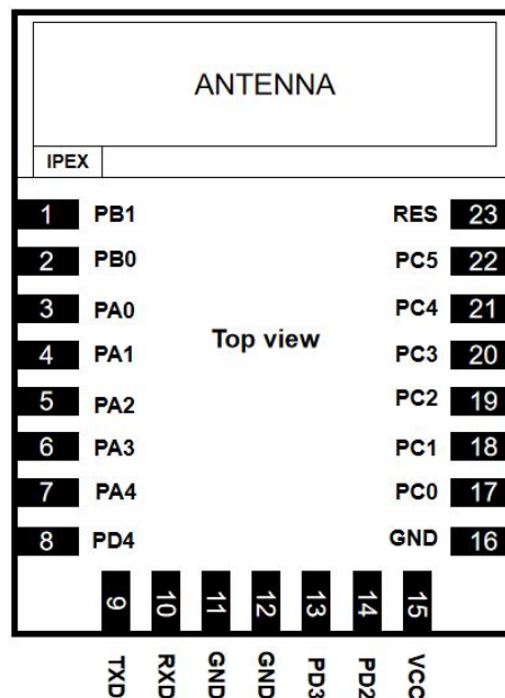
Figure 3: SKZ306 Module Pinout
