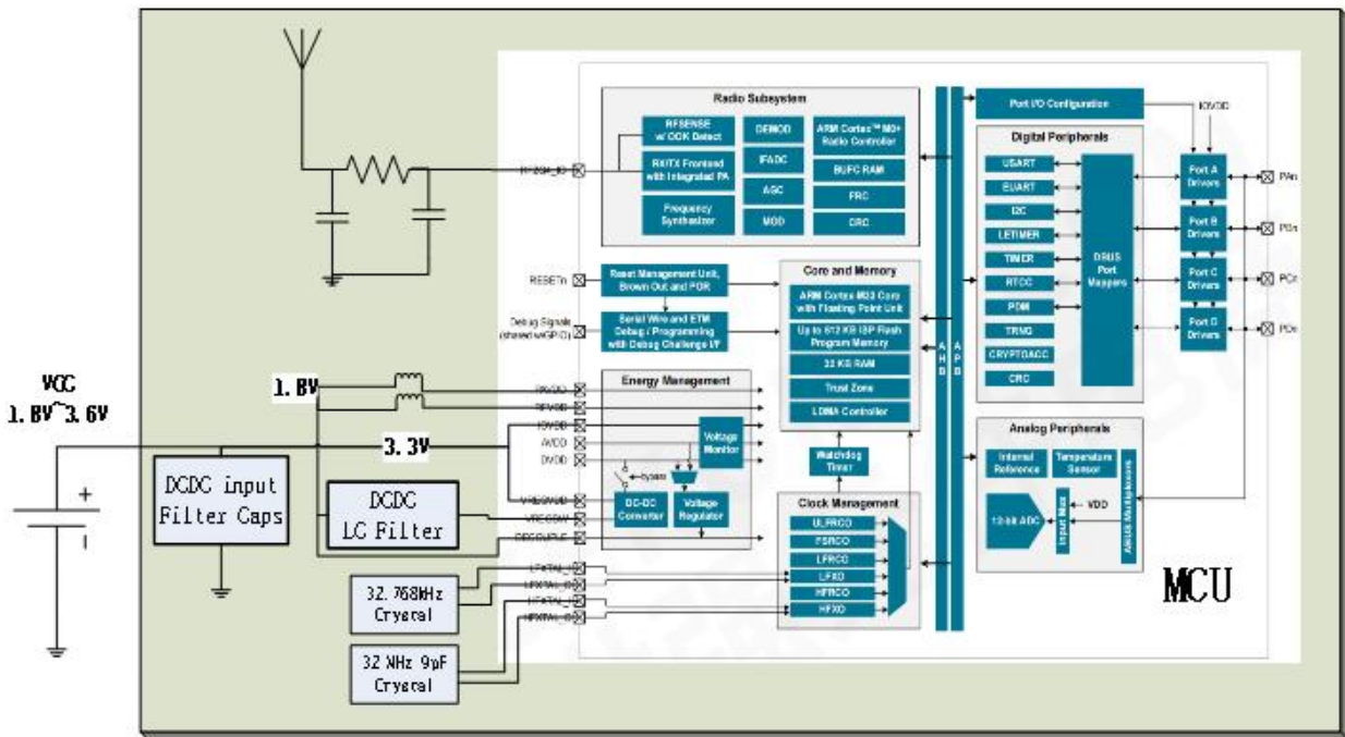
Figure 2: SKZ306 Block Diagram
