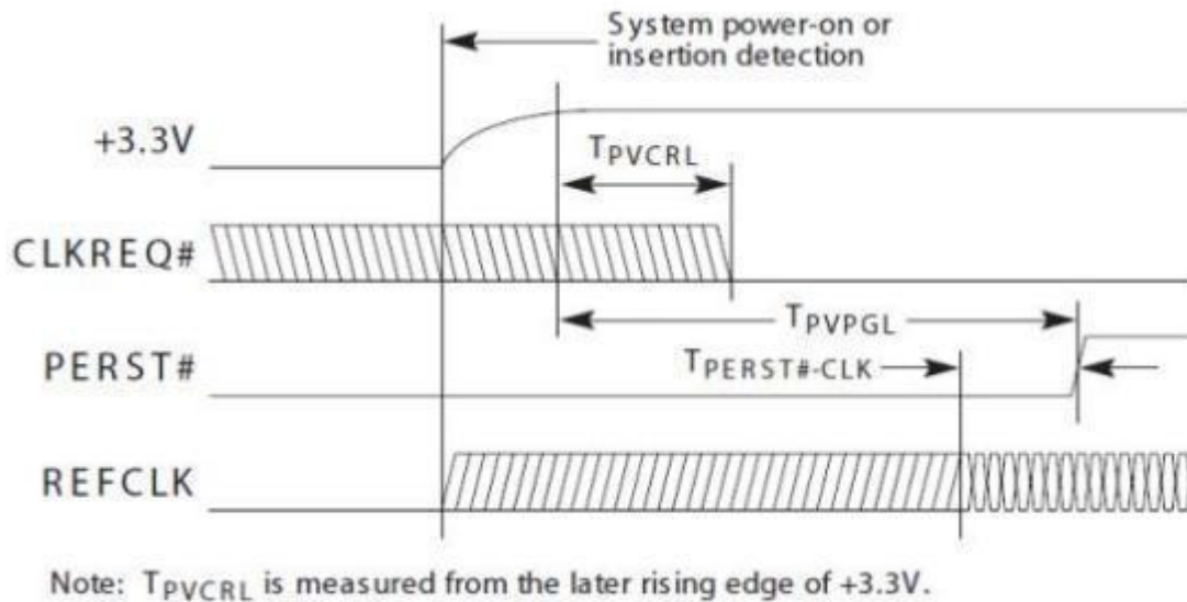
Figure 4- 1 Power up timing requirements
