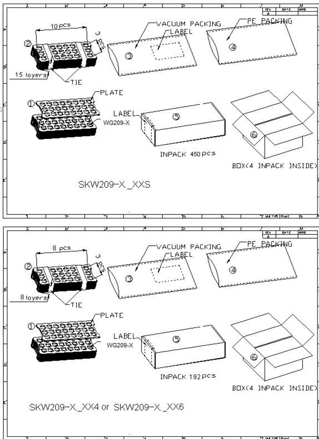
Figure 5: WG209-X Packaging
