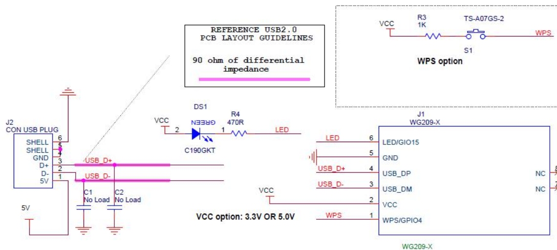
Figure 5: WG209-X schematic application
