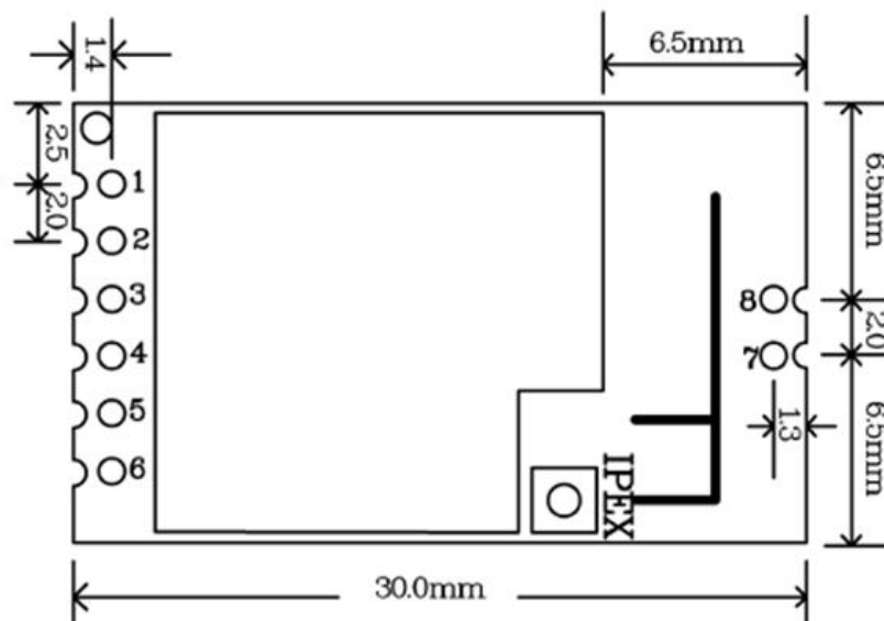
Figure 4: WG209-X Dimensions
