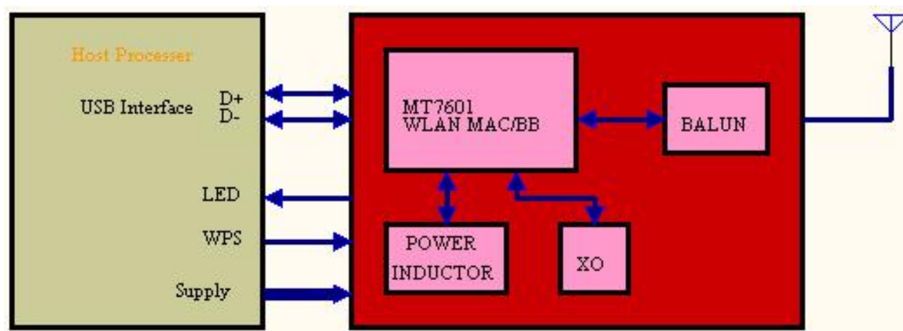
Figure 2: WG209-X Block Diagram
