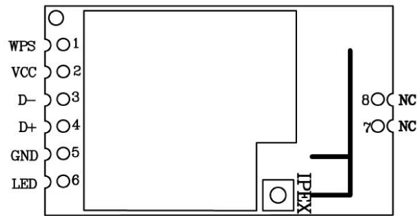
Figure 3: WG209-X Pin Name (top view)
