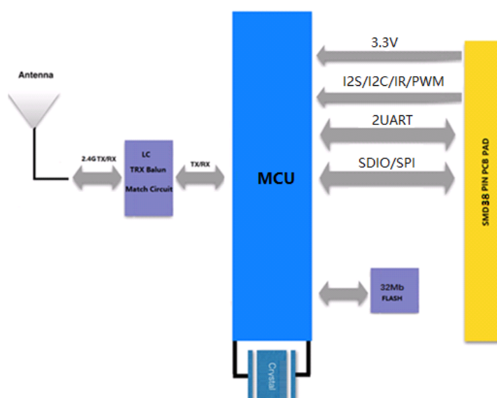
Figure 2: WG219 Block Diagram
