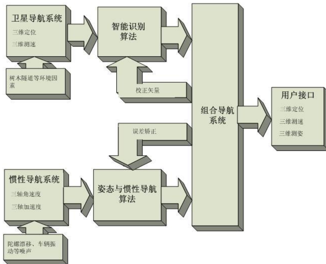
图 3: SKM2505NRD-40MXT 设计原理框图/Design diagram
