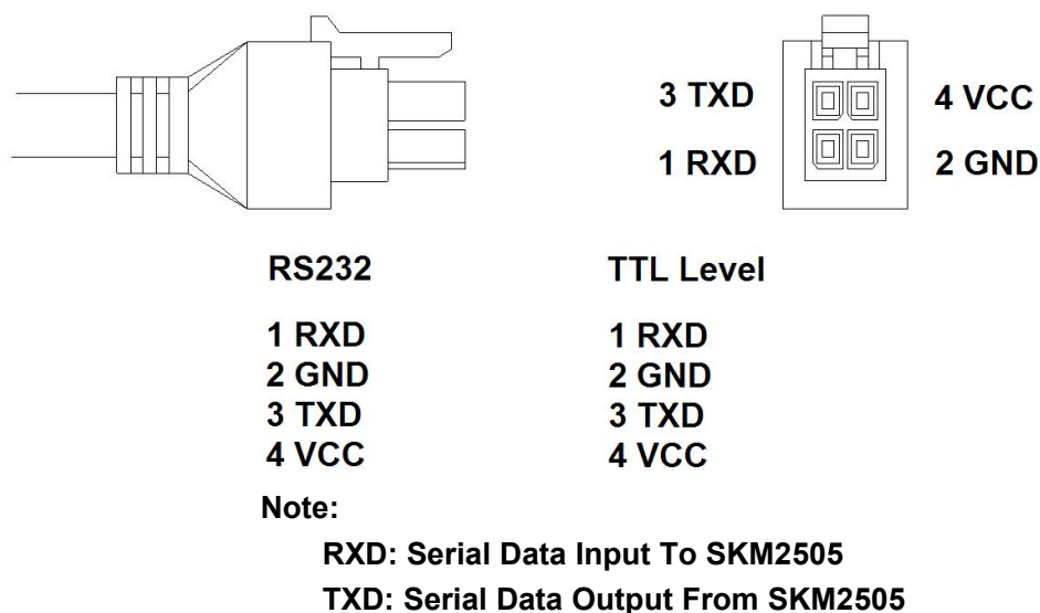
图 2: SKM2505NRD-40MXT 接口定义/Interface definition
